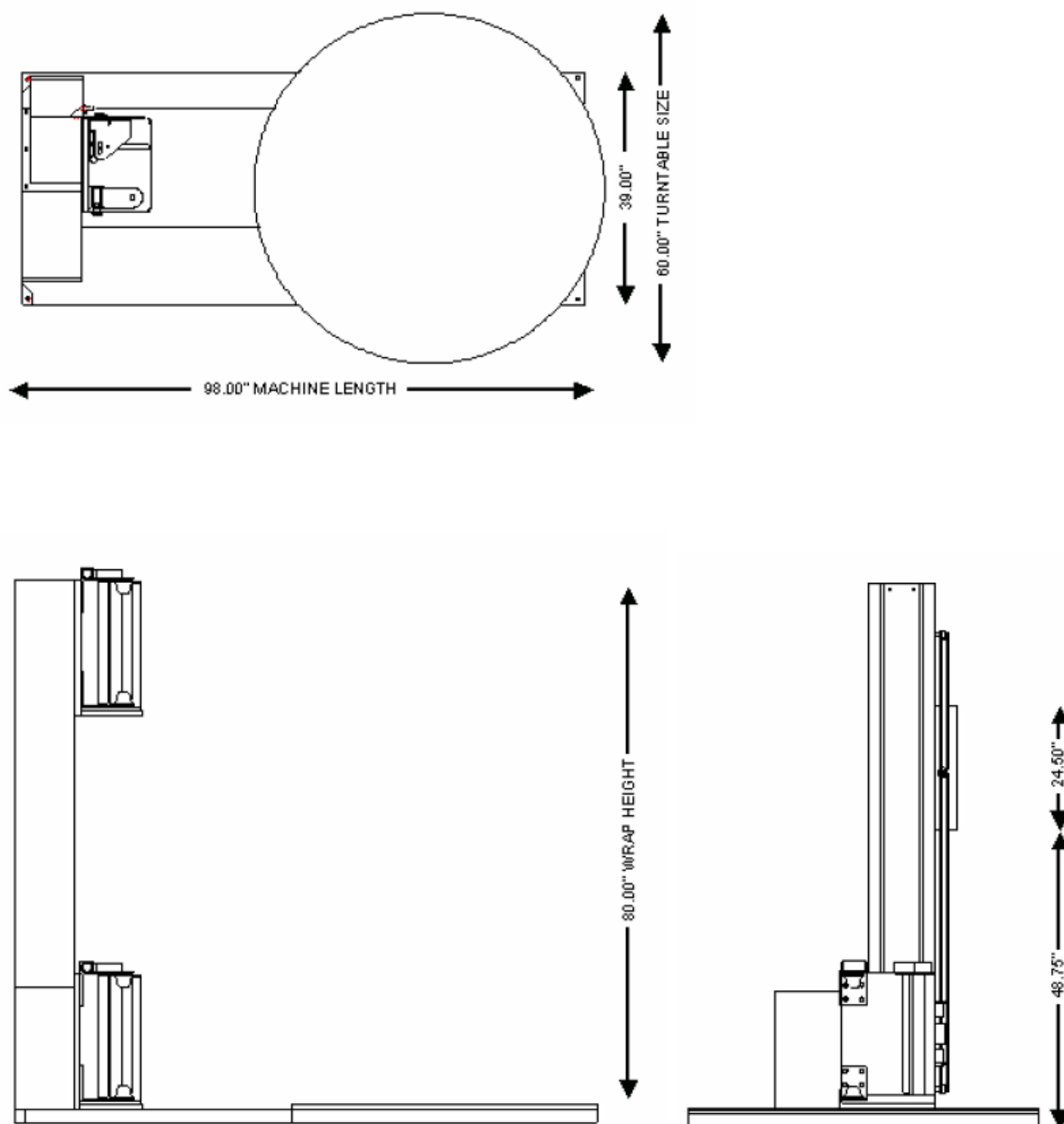
Figure 1A: Predator SS Low Profile Scale Overview Layout
